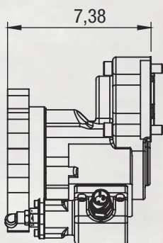
F-G Type Output SAE-C & SAE-CC 2 or 4-Bolt Flange
