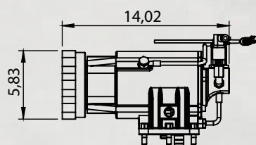
F-G Type Output SAE-C & SAE-CC 2 or 4-Bolt Flange
