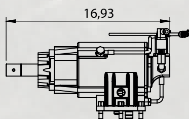
C Type Output 1 1/4" Round Keyed Shaft
